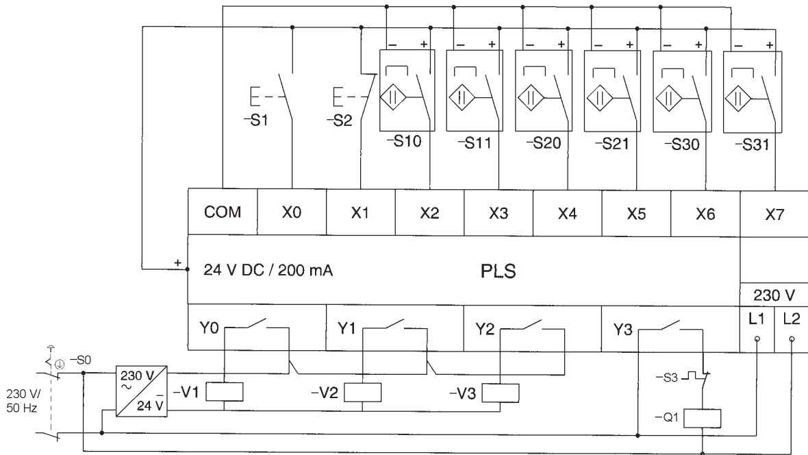
Figur 15.20 PLS-tilkoblinger
