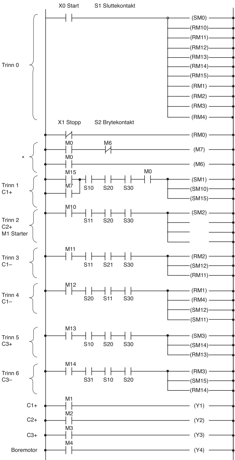
Figur 15.22 Ladderdiagram
