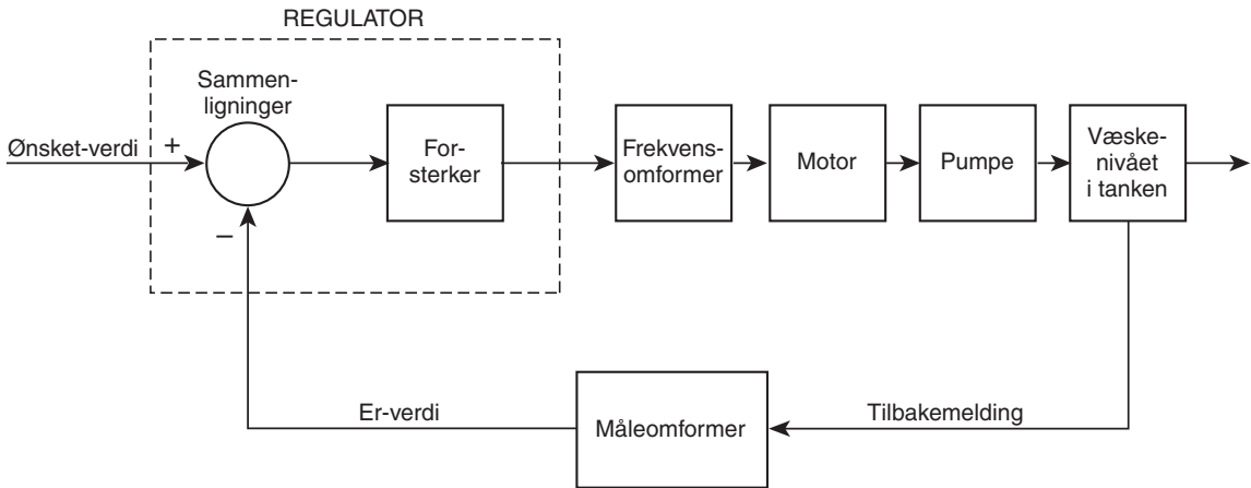
Figur 9.4 Reguleringsloyfa
