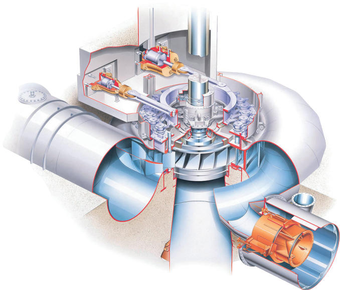
Figur 7.2 Turbin
